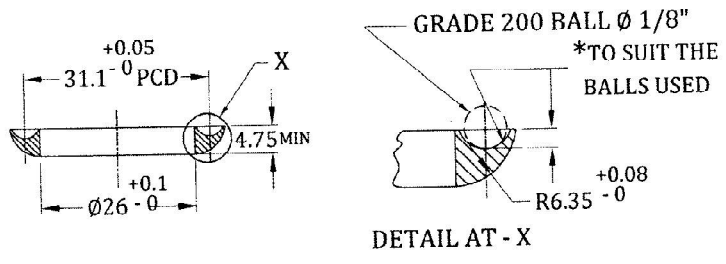
TOP AND BOTTOM INNER BALL RACE
