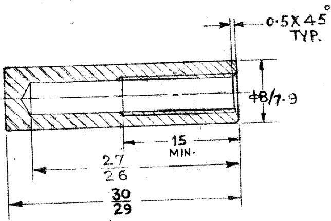
SECTION-X X
